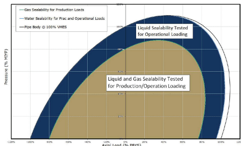
TEC-LOCK™ Wedge Coupled with SealLube™ Thread Sealant Product Family Performance
